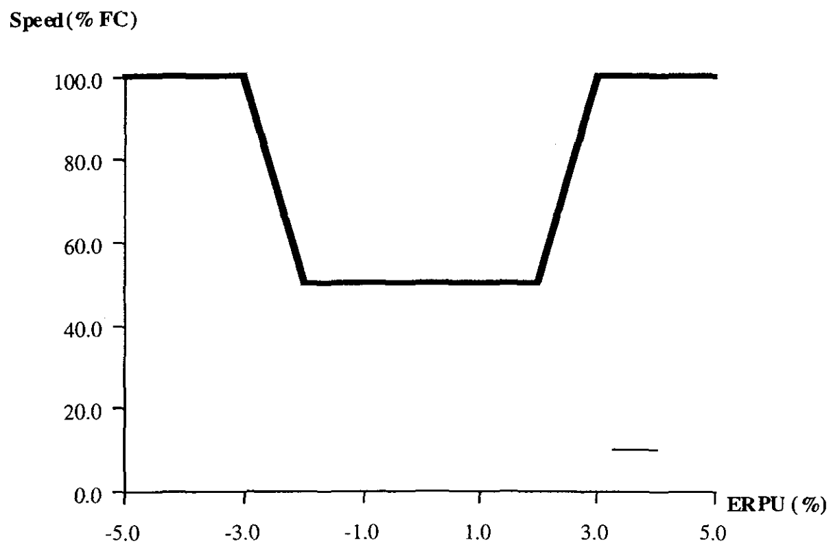
Figure 6.2: Adjuster Speed Calculation
